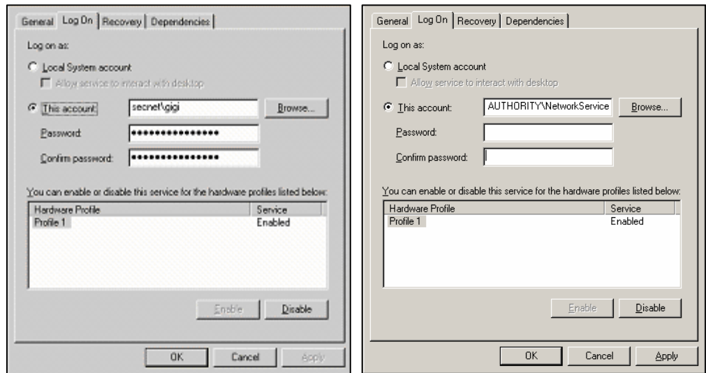
Figure B-8: Authentication Details
