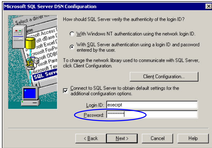
Figure 8-3: Microsoft SQL Server DSN Configuration
