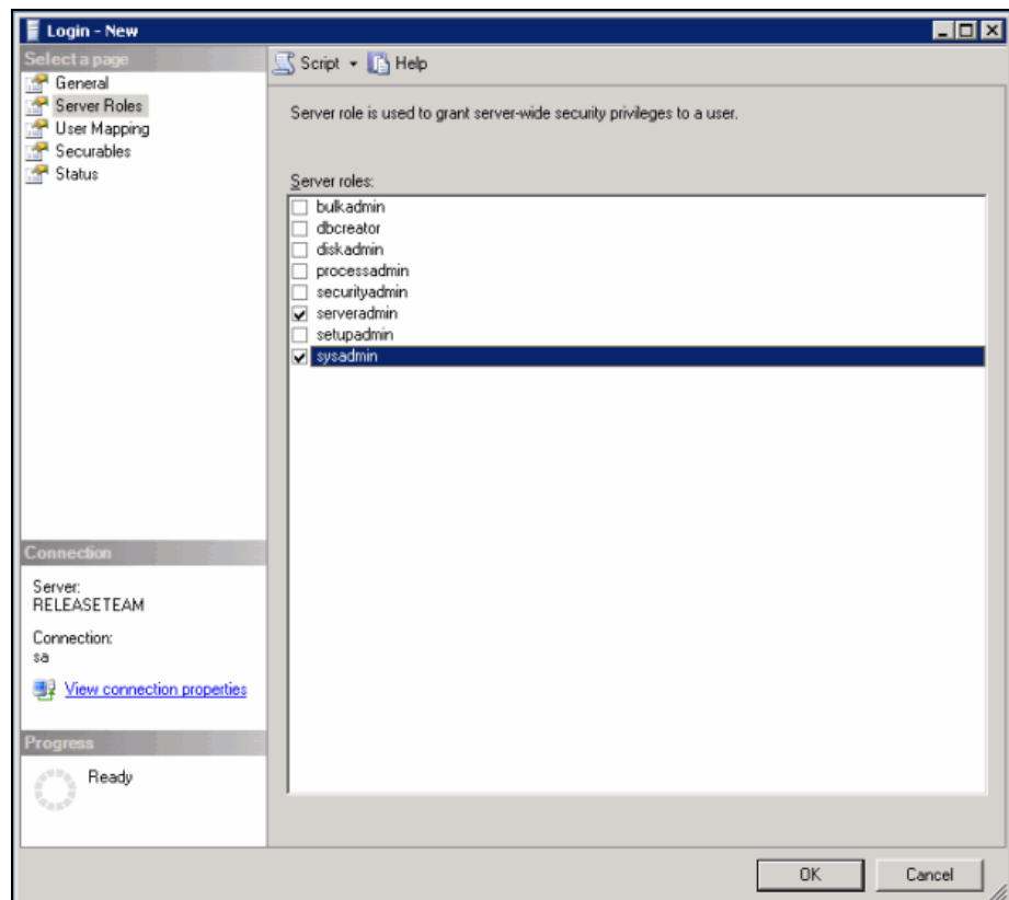
Figure B-5: Login-New- Selection of Server Roles
