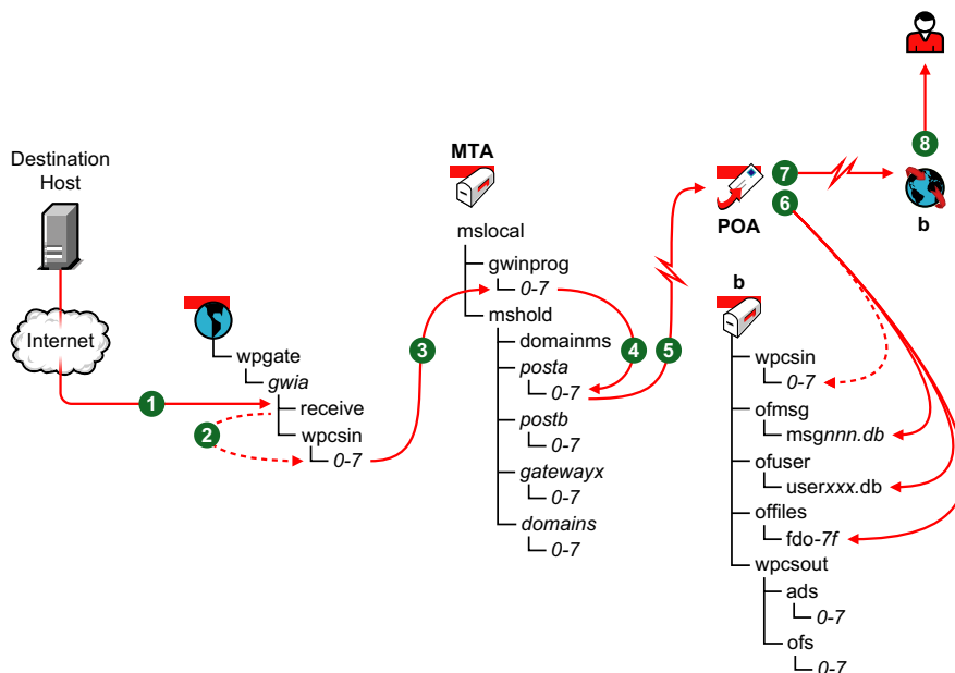
Figure 4-6 Message Flow in From the Internet
