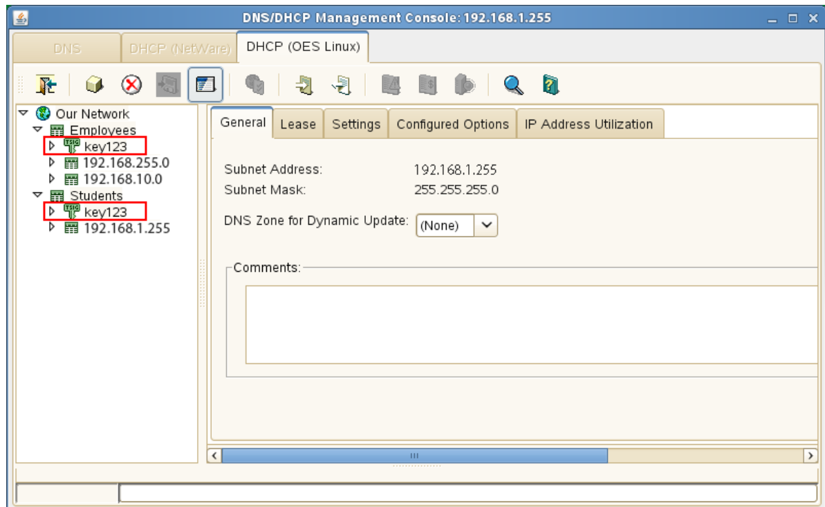
Figure 18-1 Unique keyname for services
