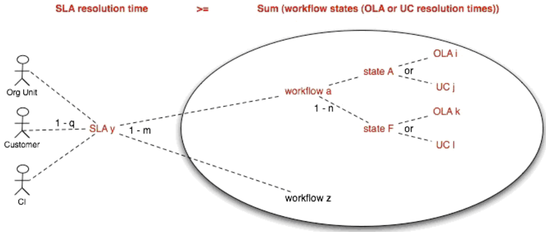
ITIL Processes - Incident, Problem or Change Management
