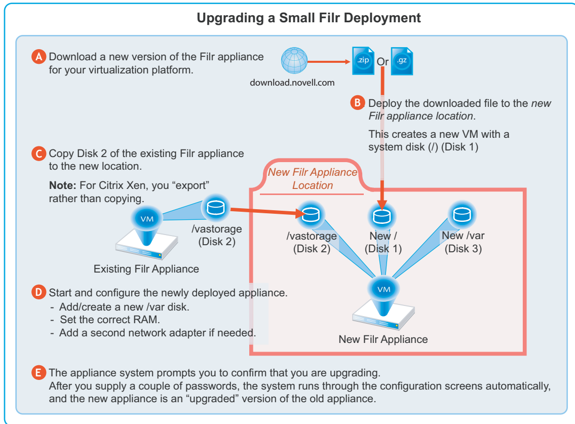
Figure 10-2 Overview of the Small Filr Appliance Upgrade Process
