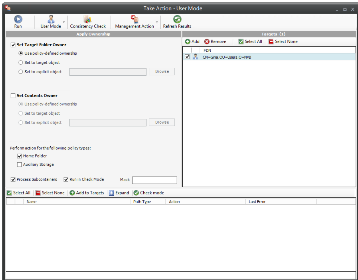
Figure 9-4 Apply Ownership Management Action Page
