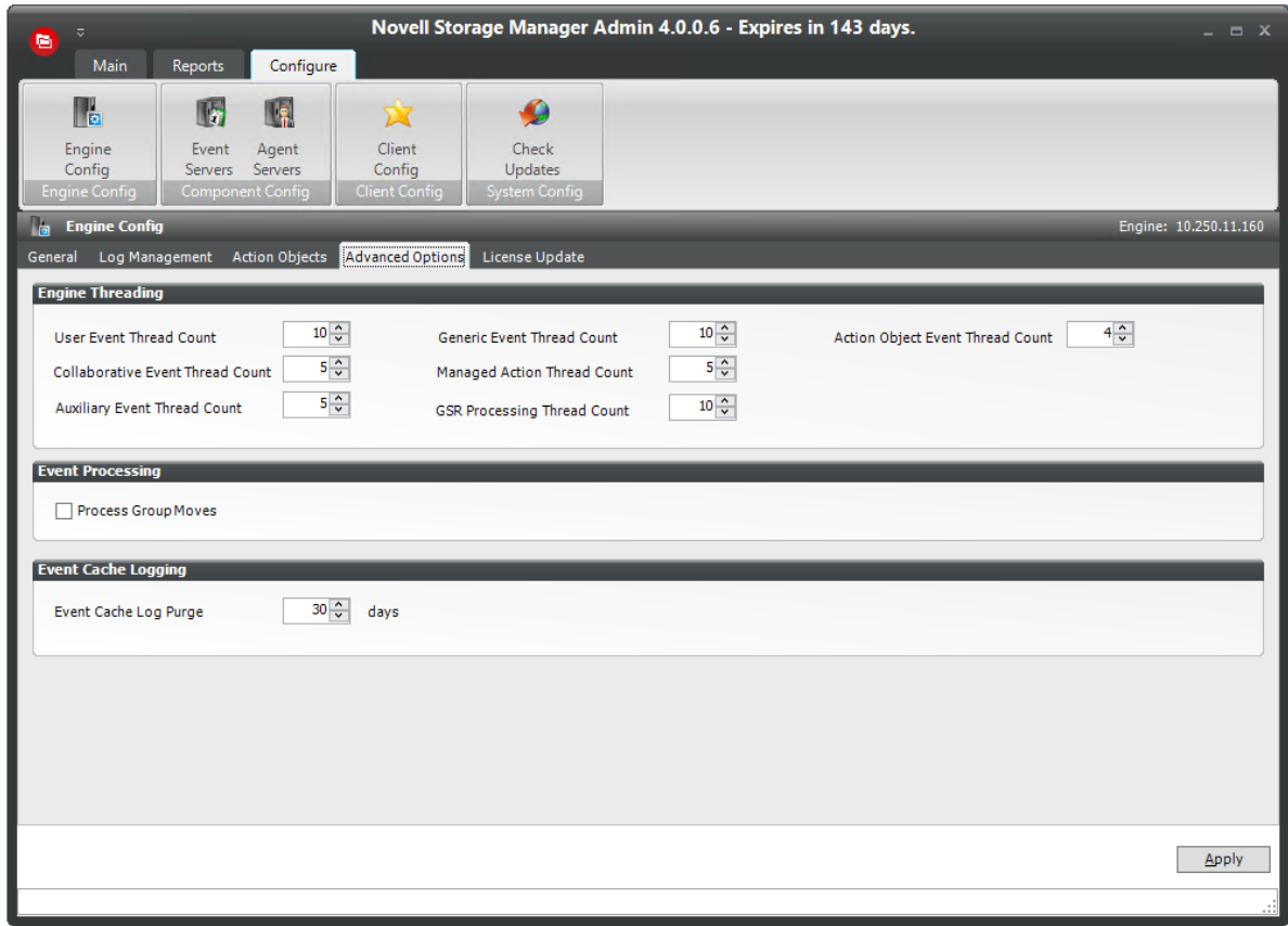
Figure 9-17 Engine Config Advanced Options Tab Settings
