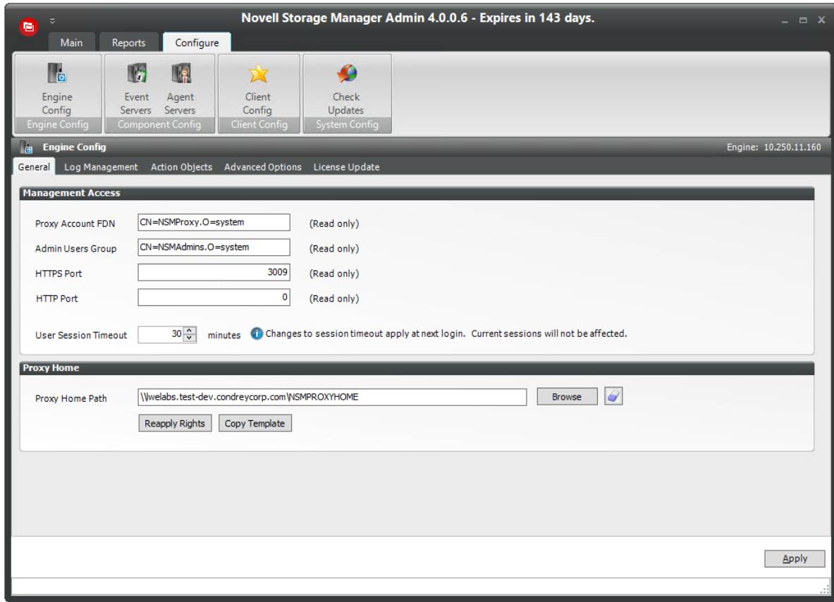
Figure 9-15 Engine Config General Tab Settings
