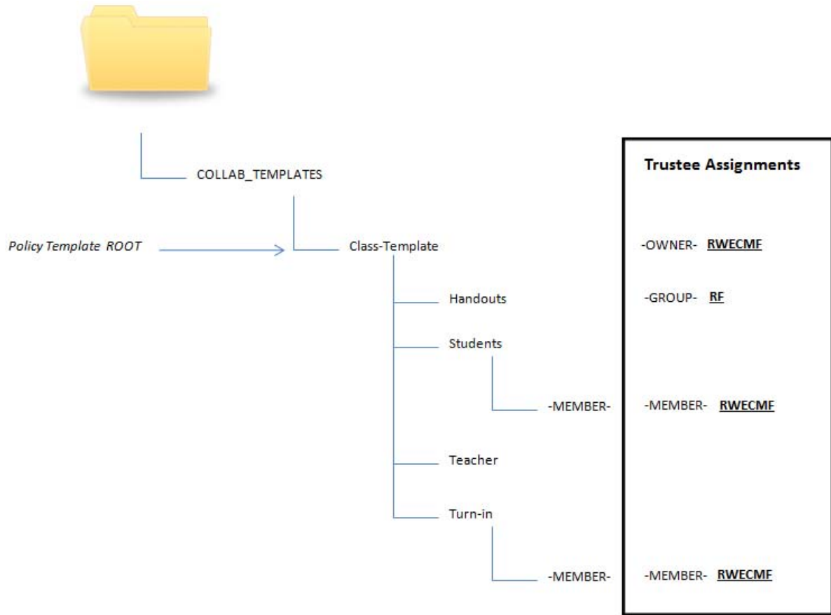
Figure 7-3 Security Permissions for Each Folder in the Sample Template
