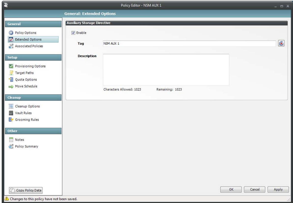
Figure B-1 Extended Options Page of an Auxiliary Storage Policy
