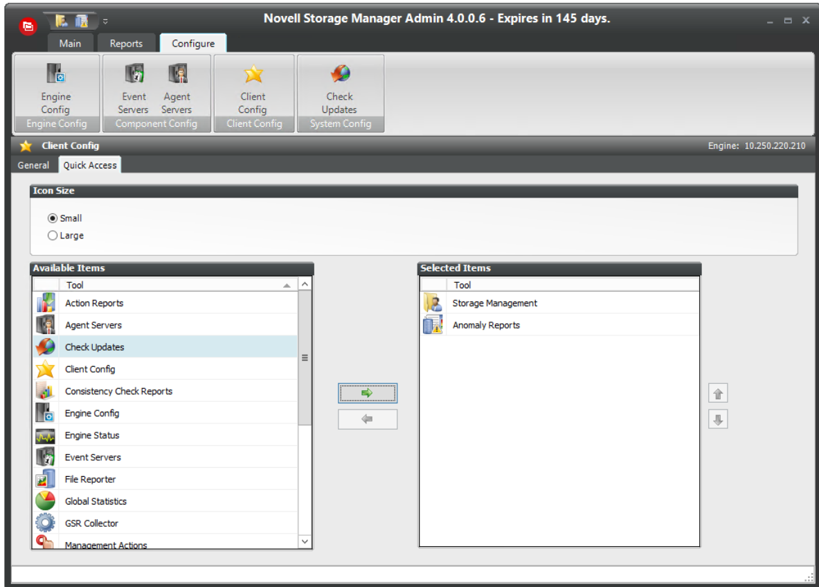
Figure 9-19 Client Config Quick Access Tab
