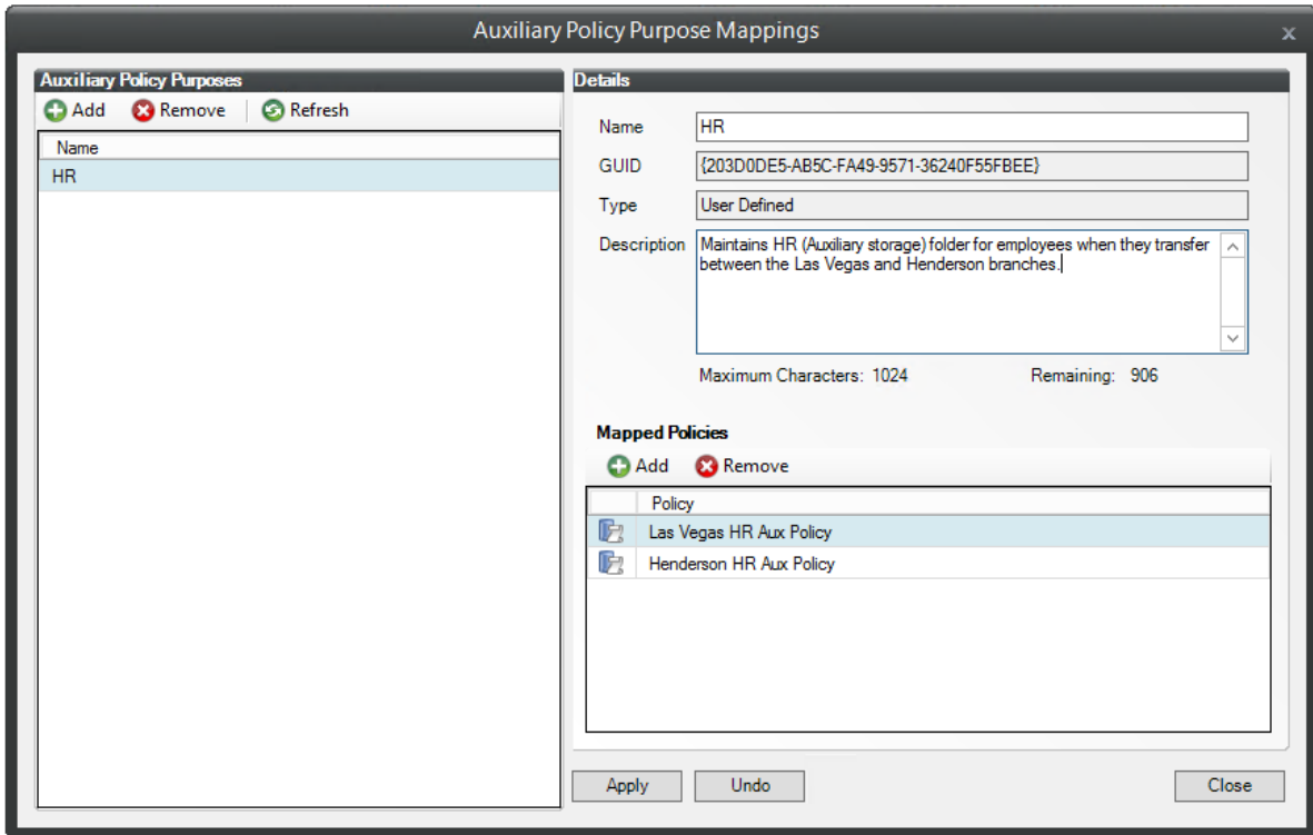
Figure 9-6 Auxiliary Purpose Mappings Dialog Box
