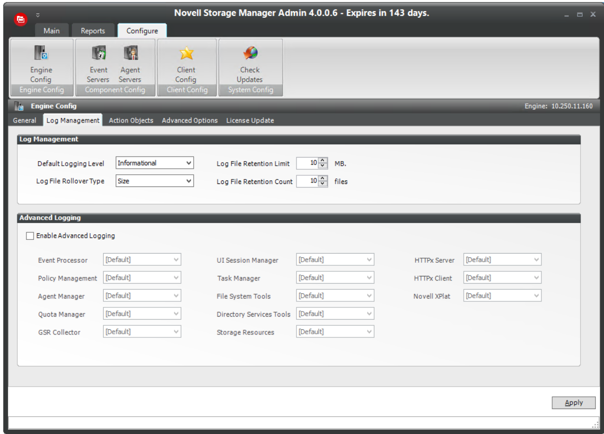
Figure 9-16 Engine Config Log Tab Settings
